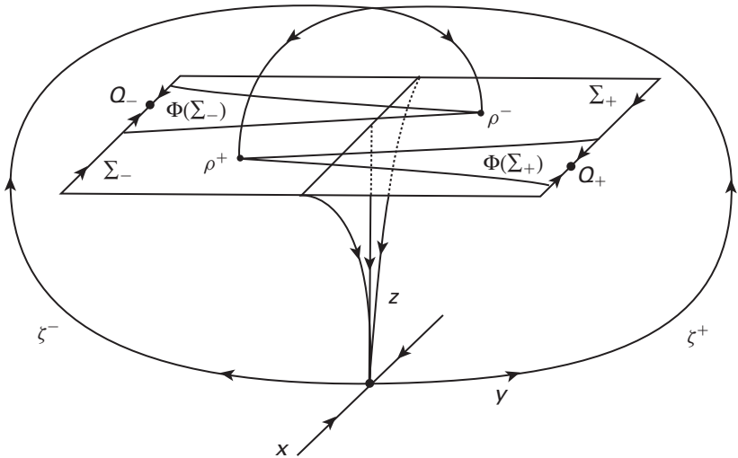
Figure 14.8 The solutions \zeta^{\pm} and their intersection with \Sigma in the model for the Lorenz attractor.
